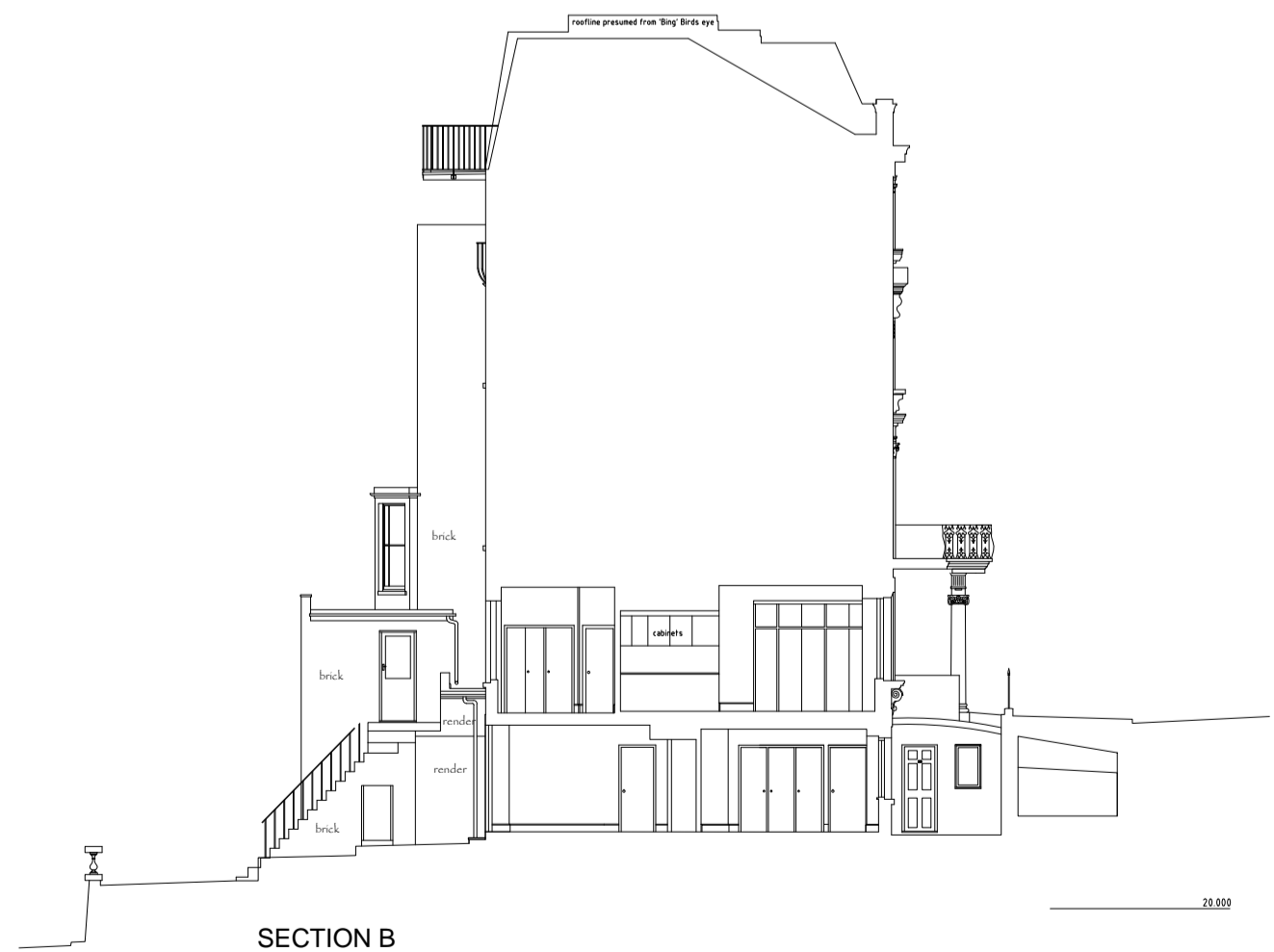
SECTION B
